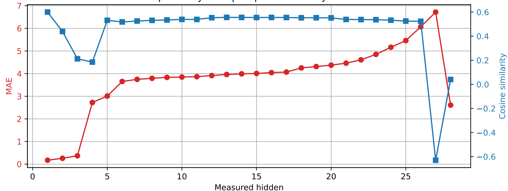
Qwen2.5-7B-Instruct | Prompt 3 Spared layer 17 | Unquantized vs hybrid
