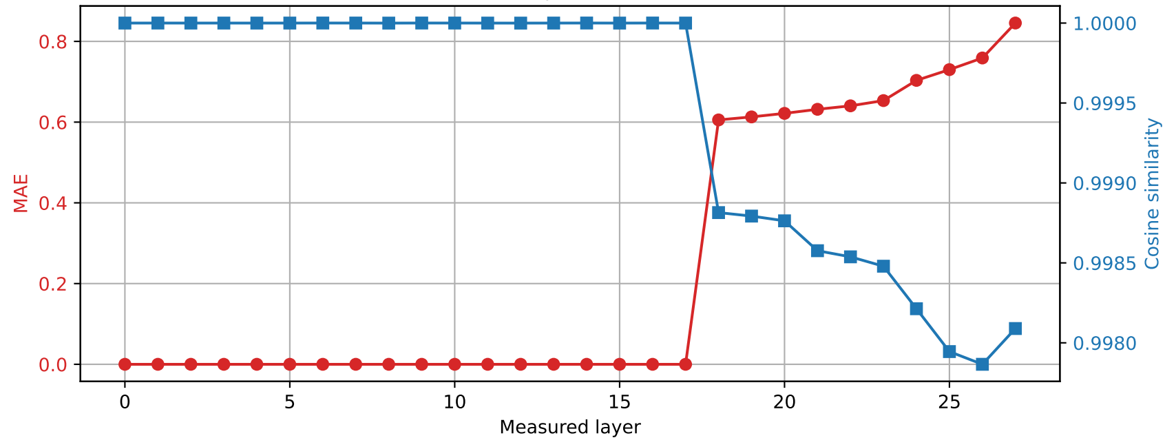
Qwen2.5-7B-Instruct | Prompt 3 Spared layer 17 | Hybrid vs quantized
