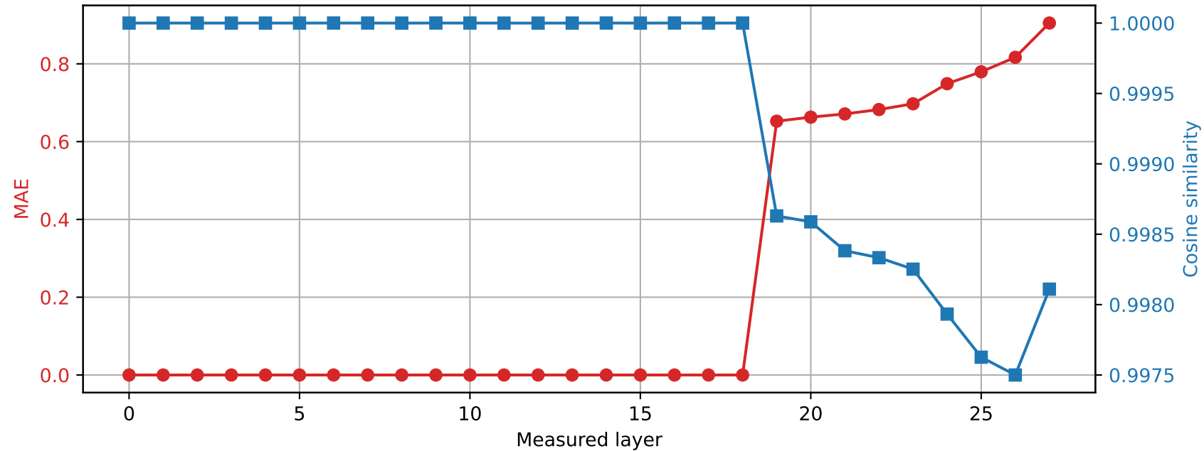
Qwen2.5-7B-Instruct | Prompt 3 Spared layer 18 | Hybrid vs quantized
