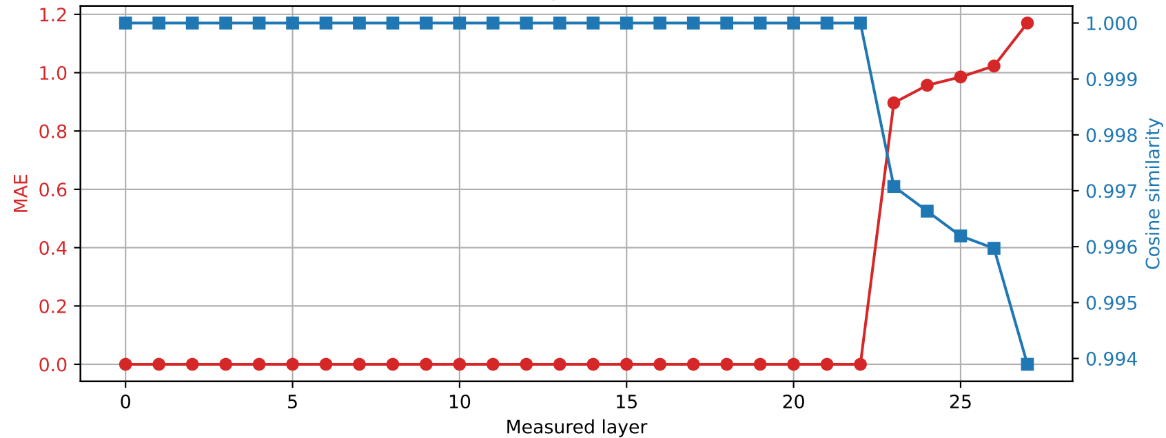
Qwen2.5-7B-Instruct | Prompt 3 Spared layer 22 | Hybrid vs quantized
