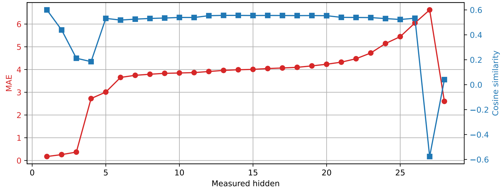
Qwen2.5-7B-Instruct | Prompt 3 Spared layer 23 | Unquantized vs hybrid
