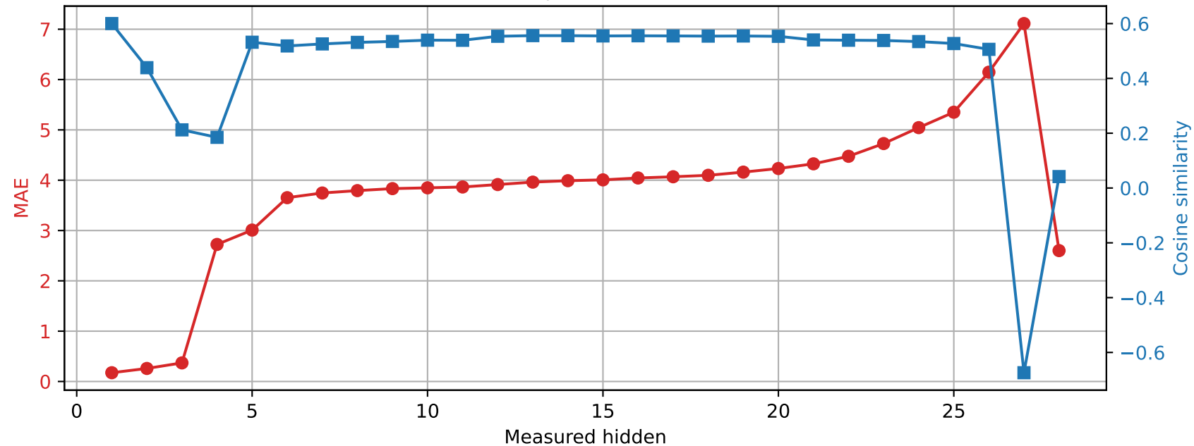
Qwen2.5-7B-Instruct | Prompt 3 Spared layer 25 | Unquantized vs hybrid
