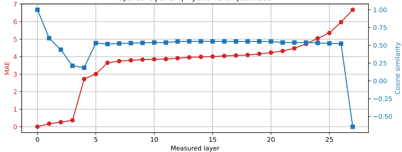
Qwen2.5-7B-Instruct | Prompt 3 Spared layer 27 | Hybrid vs unquantized
