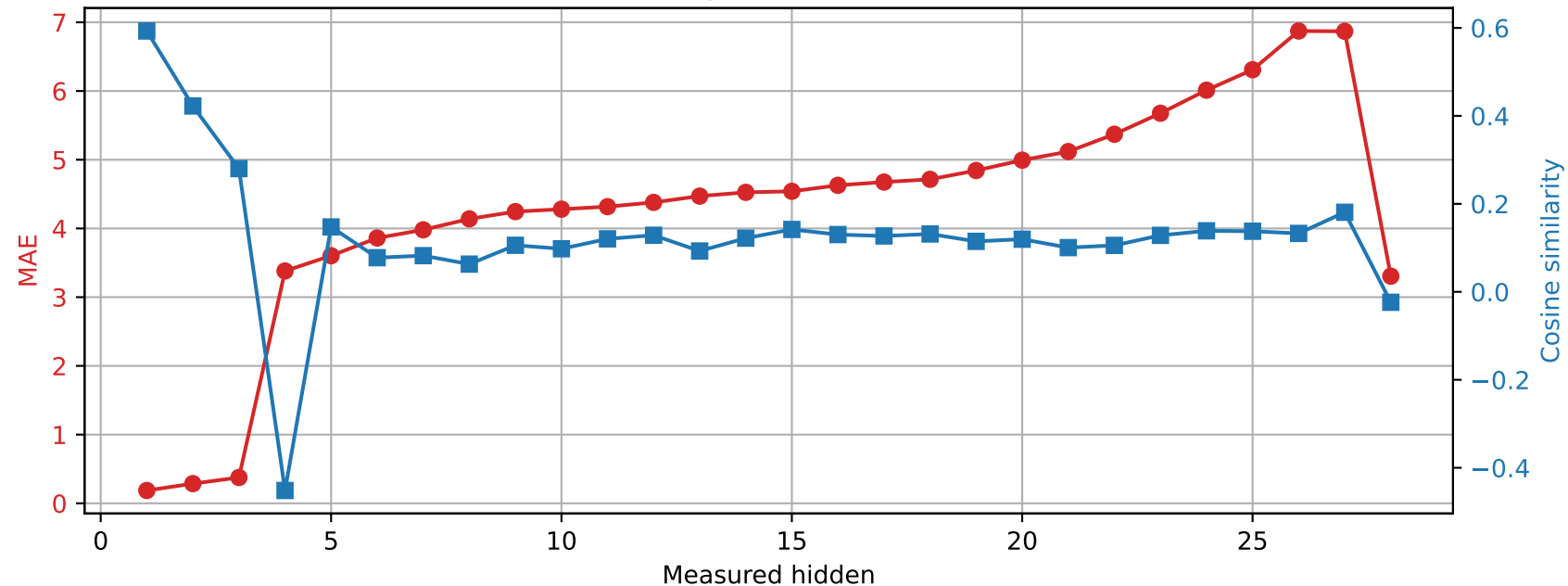
Qwen2.5-7B-Instruct | Prompt 4 Spared layer 4 | Unquantized vs hybrid
