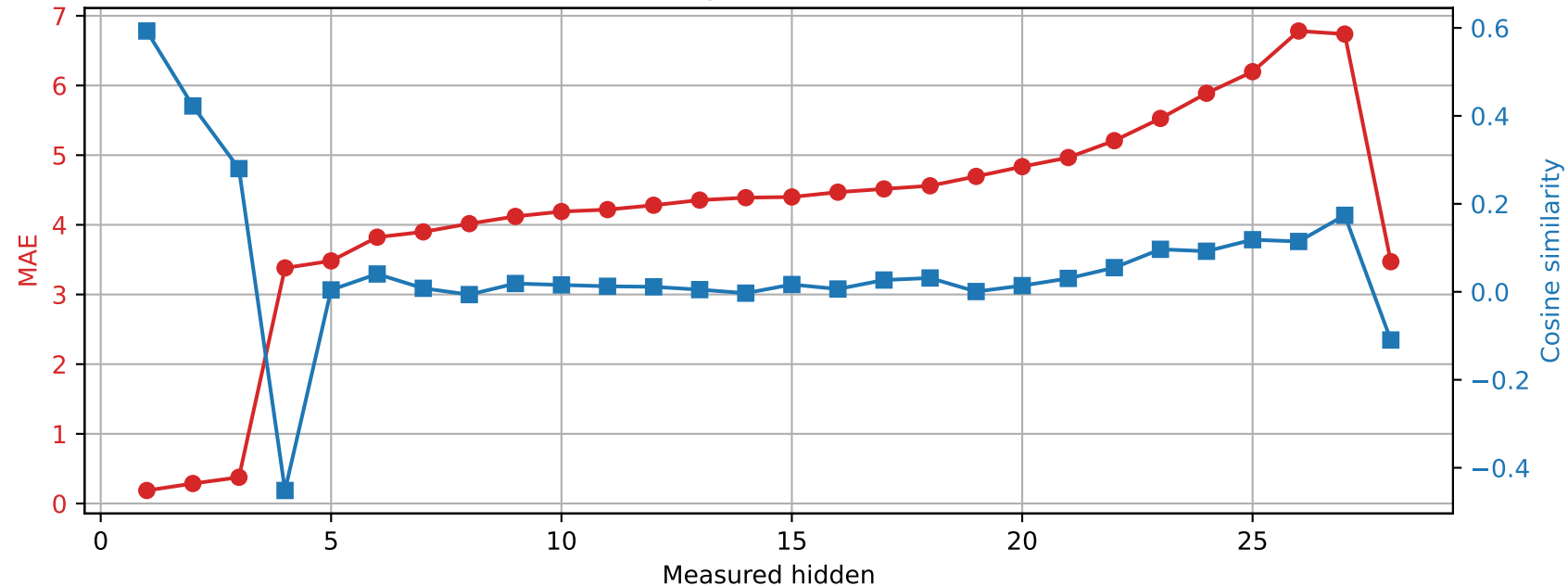
Qwen2.5-7B-Instruct | Prompt 4 Spared layer 5 | Unquantized vs hybrid
