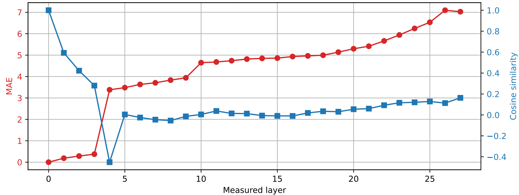
Qwen2.5-7B-Instruct | Prompt 4 Spared layer 9 | Hybrid vs unquantized
