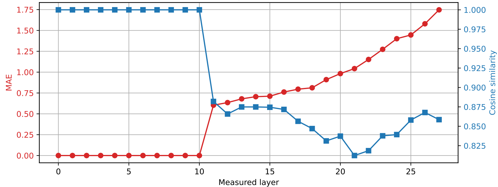
Qwen2.5-7B-Instruct | Prompt 4 Spared layer 10 | Hybrid vs quantized
