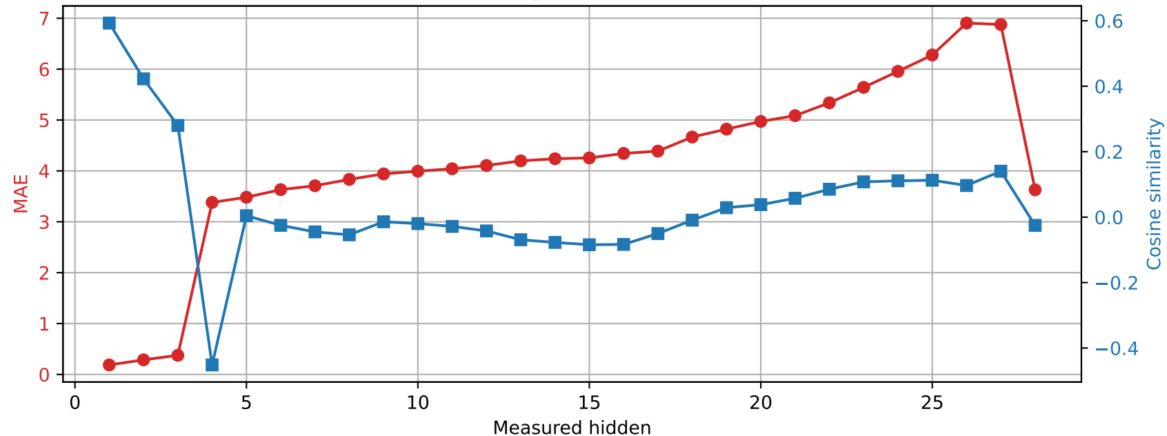
Qwen2.5-7B-Instruct | Prompt 4 Spared layer 17 | Unquantized vs hybrid
