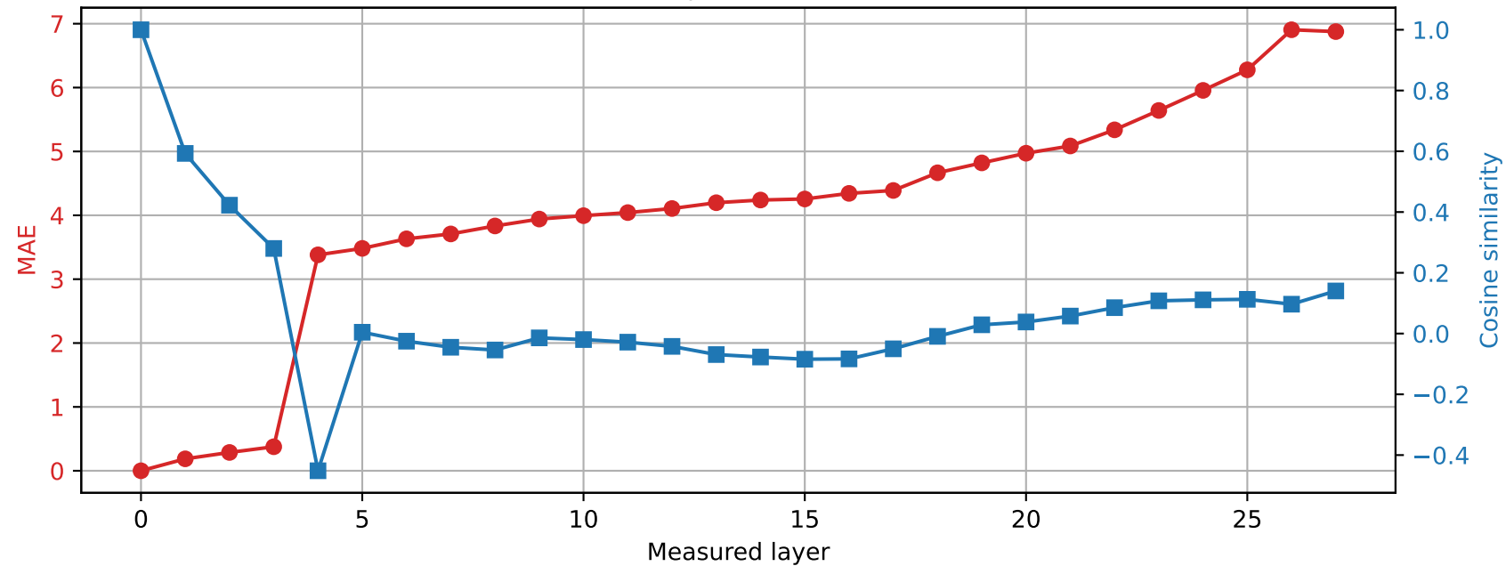
Qwen2.5-7B-Instruct | Prompt 4 Spared layer 17 | Hybrid vs unquantized
