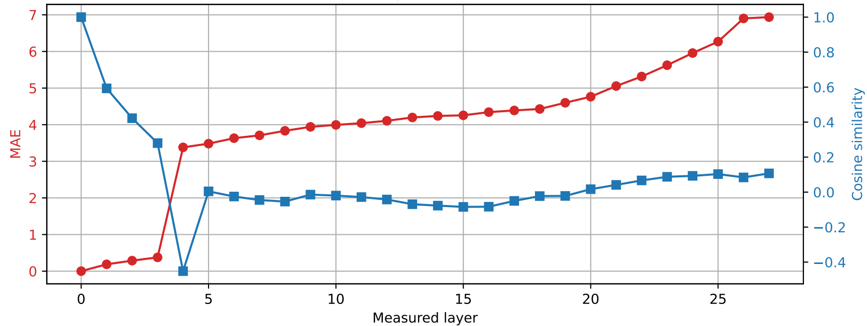
Qwen2.5-7B-Instruct | Prompt 4 Spared layer 20 | Hybrid vs unquantized
