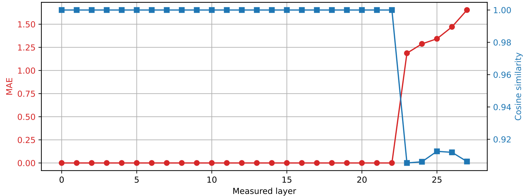
Qwen2.5-7B-Instruct | Prompt 4 Spared layer 22 | Hybrid vs quantized
