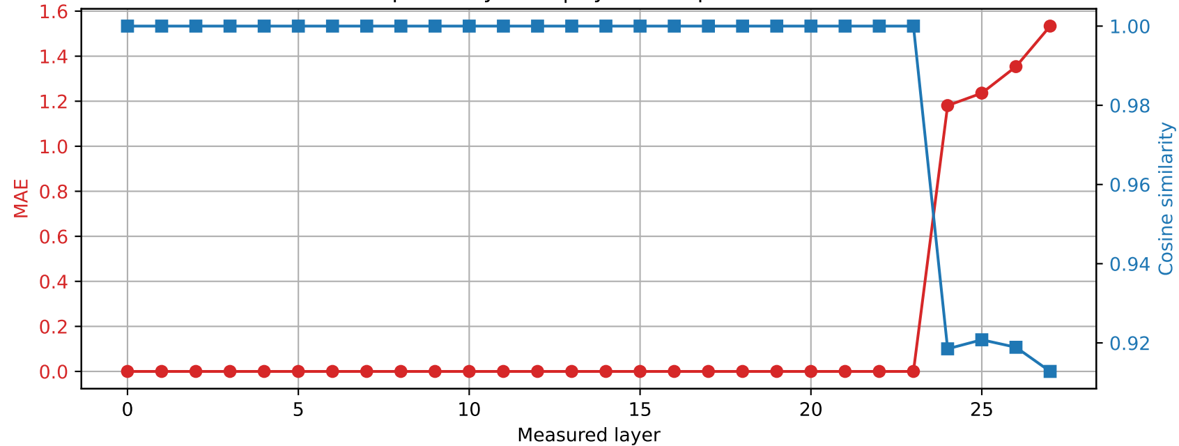
Qwen2.5-7B-Instruct | Prompt 4 Spared layer 23 | Hybrid vs quantized
