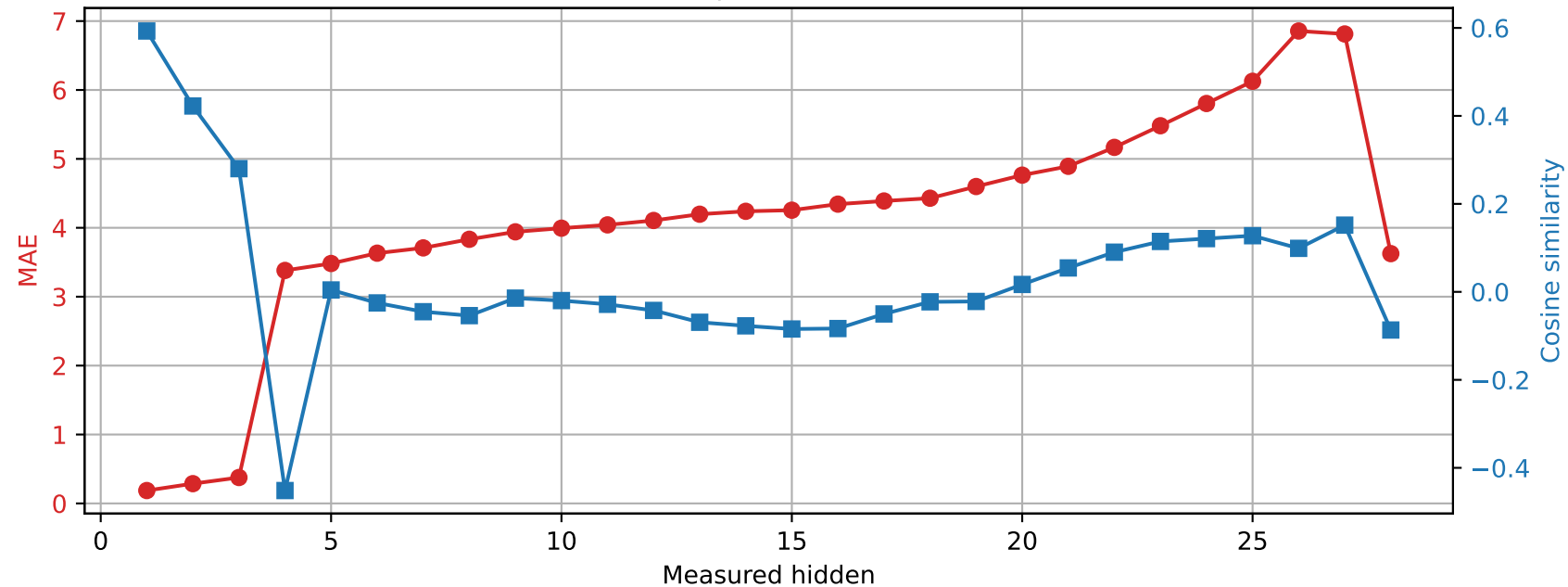
Qwen2.5-7B-Instruct | Prompt 4 Spared layer 25 | Unquantized vs hybrid
