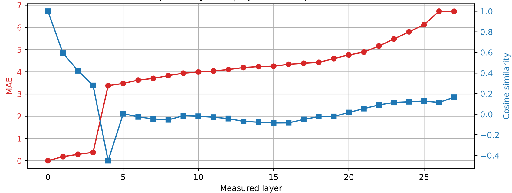
Qwen2.5-7B-Instruct | Prompt 4 Spared layer 27 | Hybrid vs unquantized
