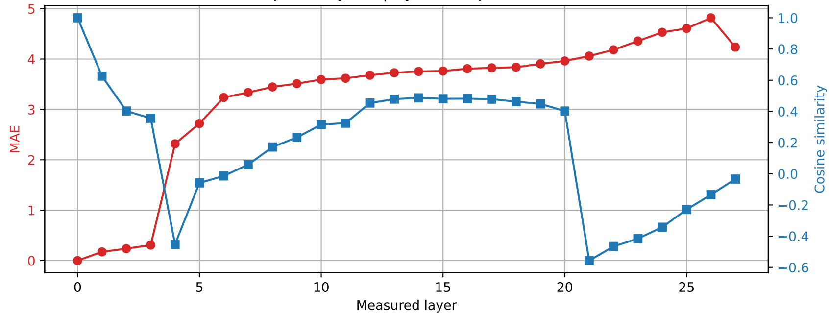
Qwen2.5-7B-Instruct | Prompt 0 Spared layer 0 | Hybrid vs quantized
