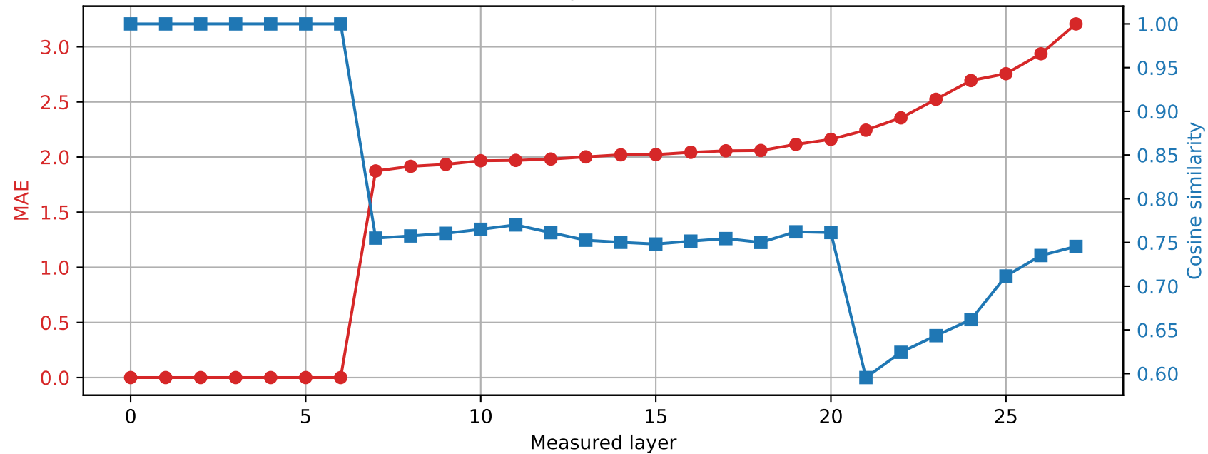
Qwen2.5-7B-Instruct | Prompt 0 Spared layer 6 | Hybrid vs quantized
