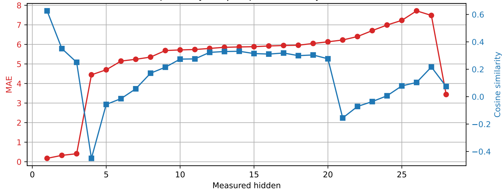
Qwen2.5-7B-Instruct | Prompt 0 Spared layer 8 | Unquantized vs hybrid
