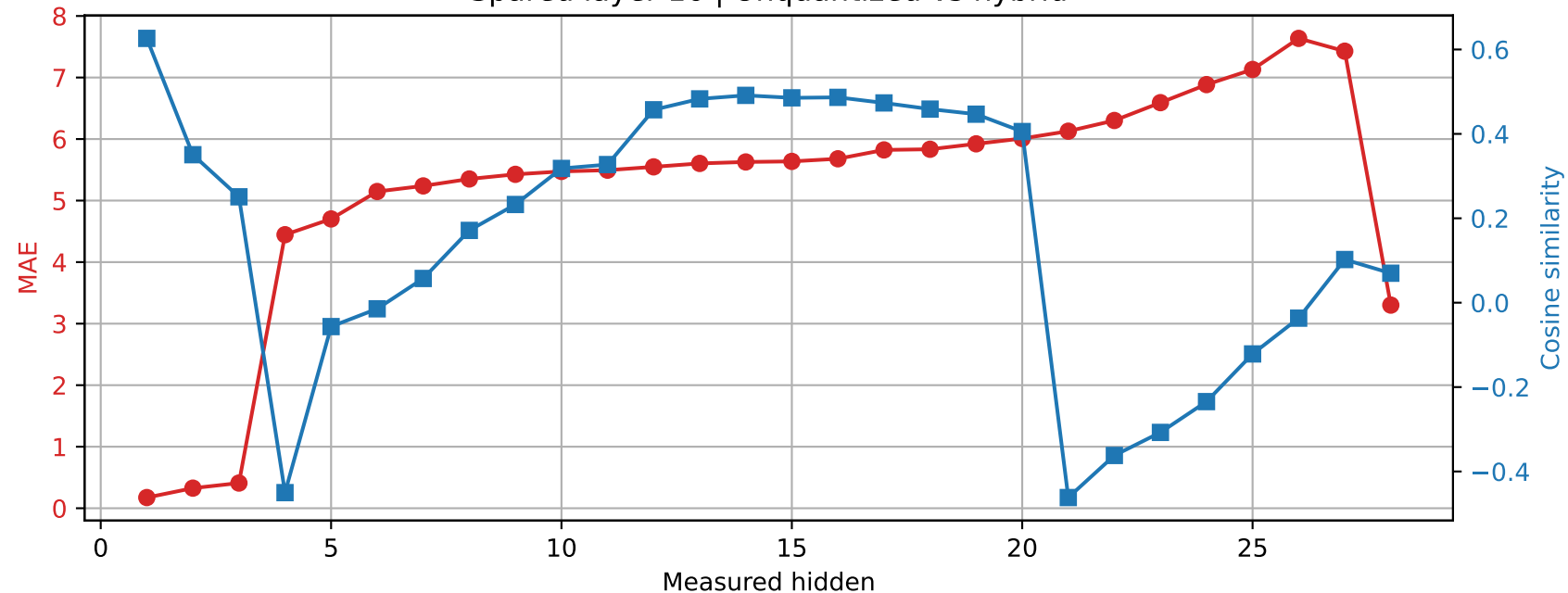
Qwen2.5-7B-Instruct | Prompt 0 Spared layer 16 | Unquantized vs hybrid
