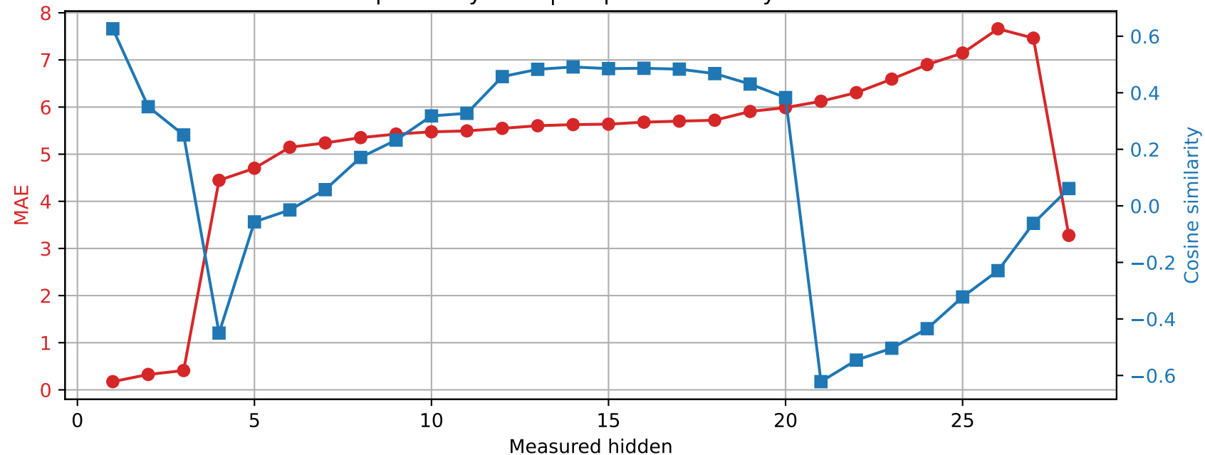
Qwen2.5-7B-Instruct | Prompt 0 Spared layer 18 | Unquantized vs hybrid
