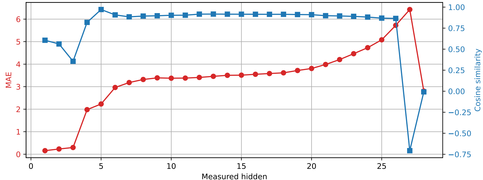
Qwen2.5-7B-Instruct | Prompt 1 Spared layer 7 | Unquantized vs hybrid
