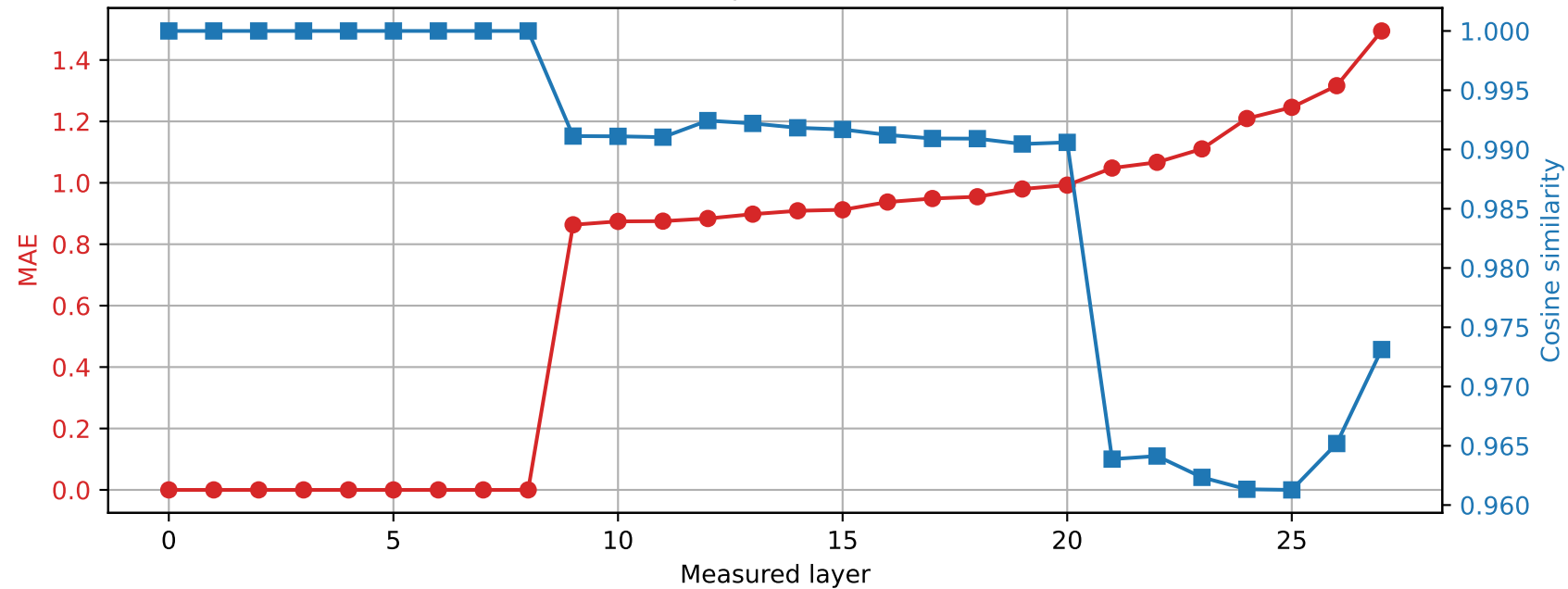
Qwen2.5-7B-Instruct | Prompt 1 Spared layer 8 | Hybrid vs quantized
