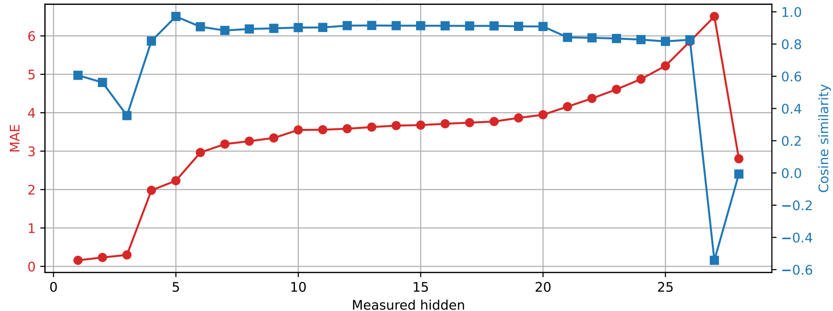
Qwen2.5-7B-Instruct | Prompt 1 Spared layer 9 | Unquantized vs hybrid
