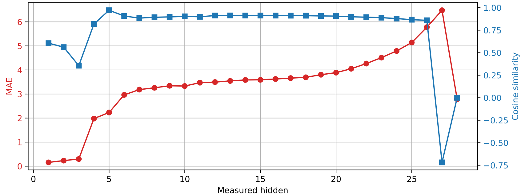
Qwen2.5-7B-Instruct | Prompt 1 Spared layer 10 | Unquantized vs hybrid
