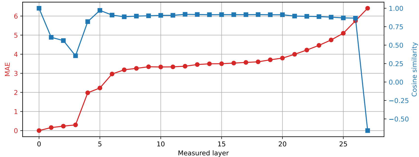
Qwen2.5-7B-Instruct | Prompt 1 Spared layer 12 | Hybrid vs unquantized
