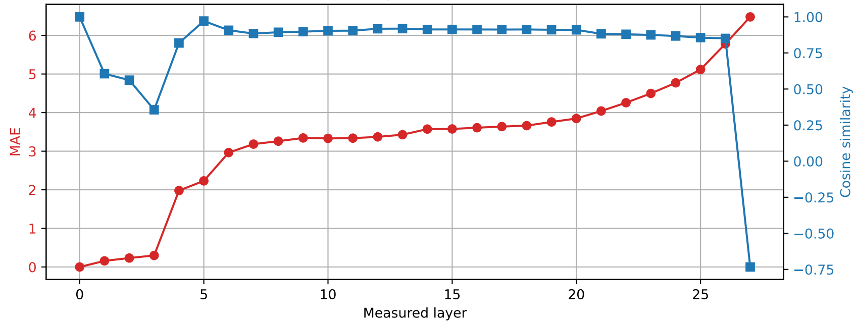
Qwen2.5-7B-Instruct | Prompt 1 Spared layer 13 | Hybrid vs unquantized
