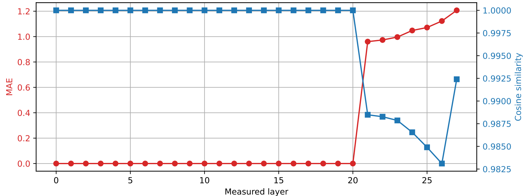
Qwen2.5-7B-Instruct | Prompt 1 Spared layer 20 | Hybrid vs quantized
