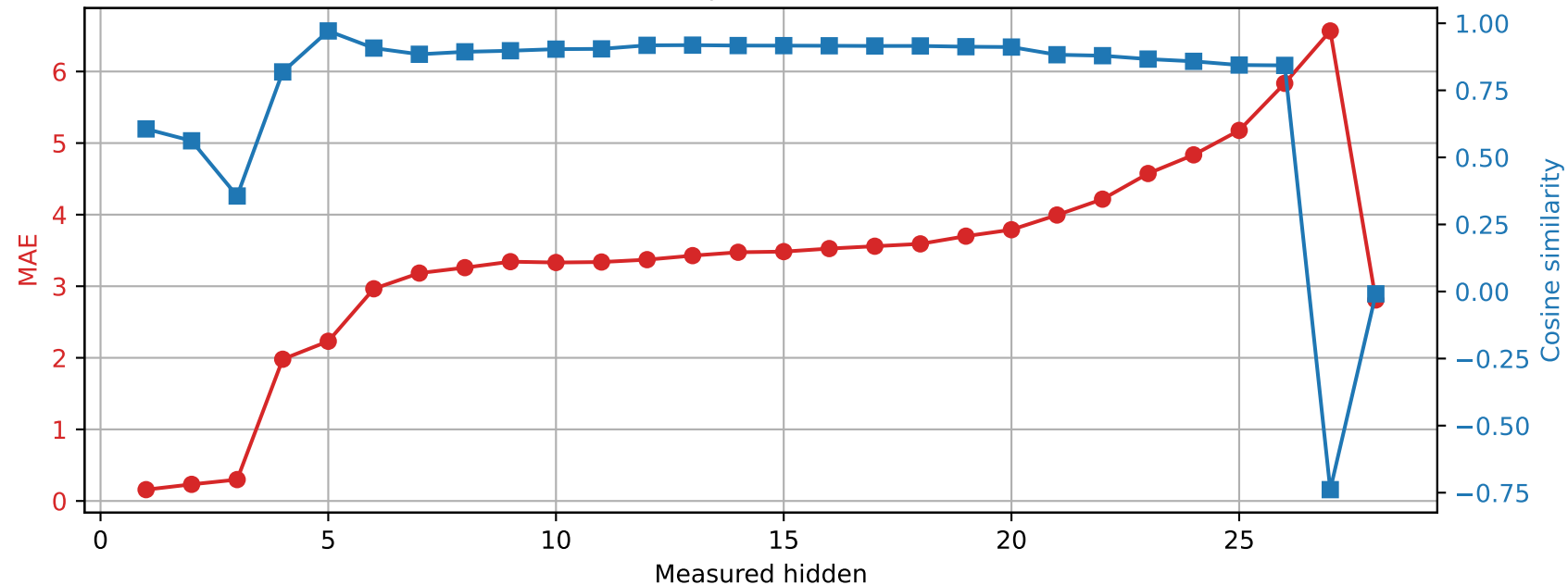
Qwen2.5-7B-Instruct | Prompt 1 Spared layer 22 | Unquantized vs hybrid
