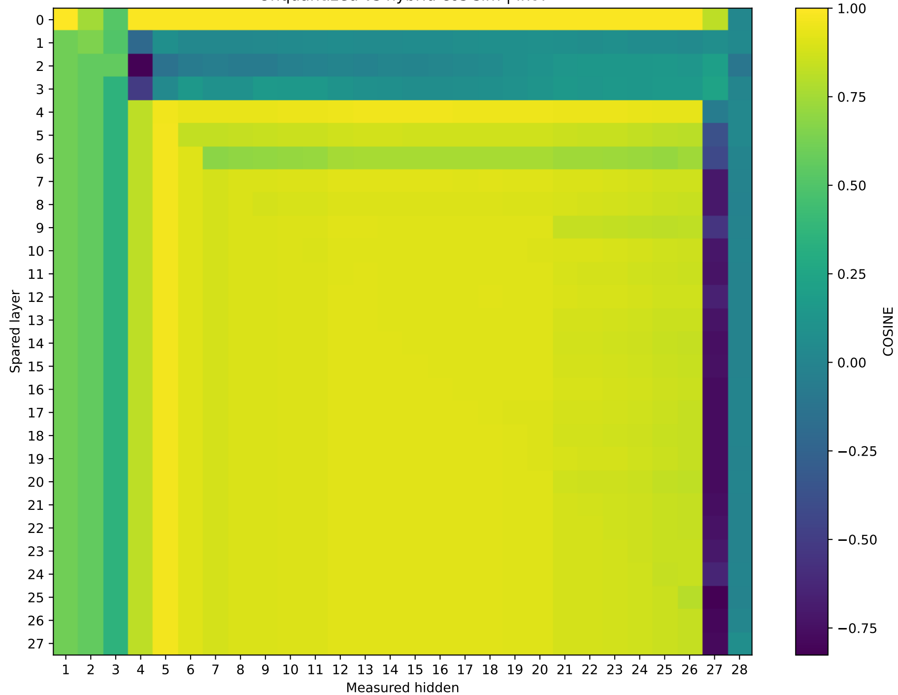
Qwen2.5-7B-Instruct | Prompt 1 Unquantized vs hybrid cos sim | int4
