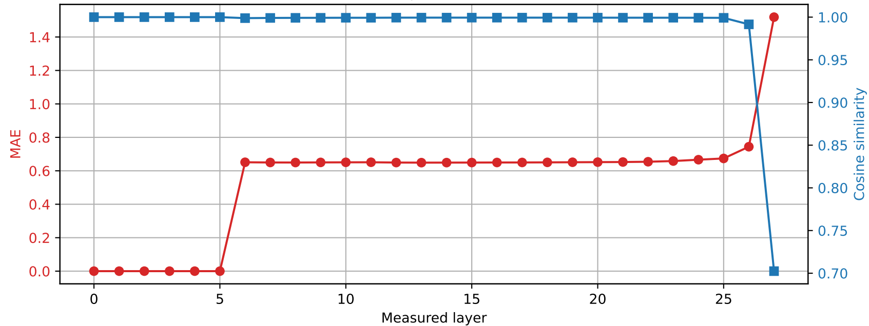
Qwen2.5-7B-Instruct | Prompt 2 Spared layer 5 | Hybrid vs quantized
