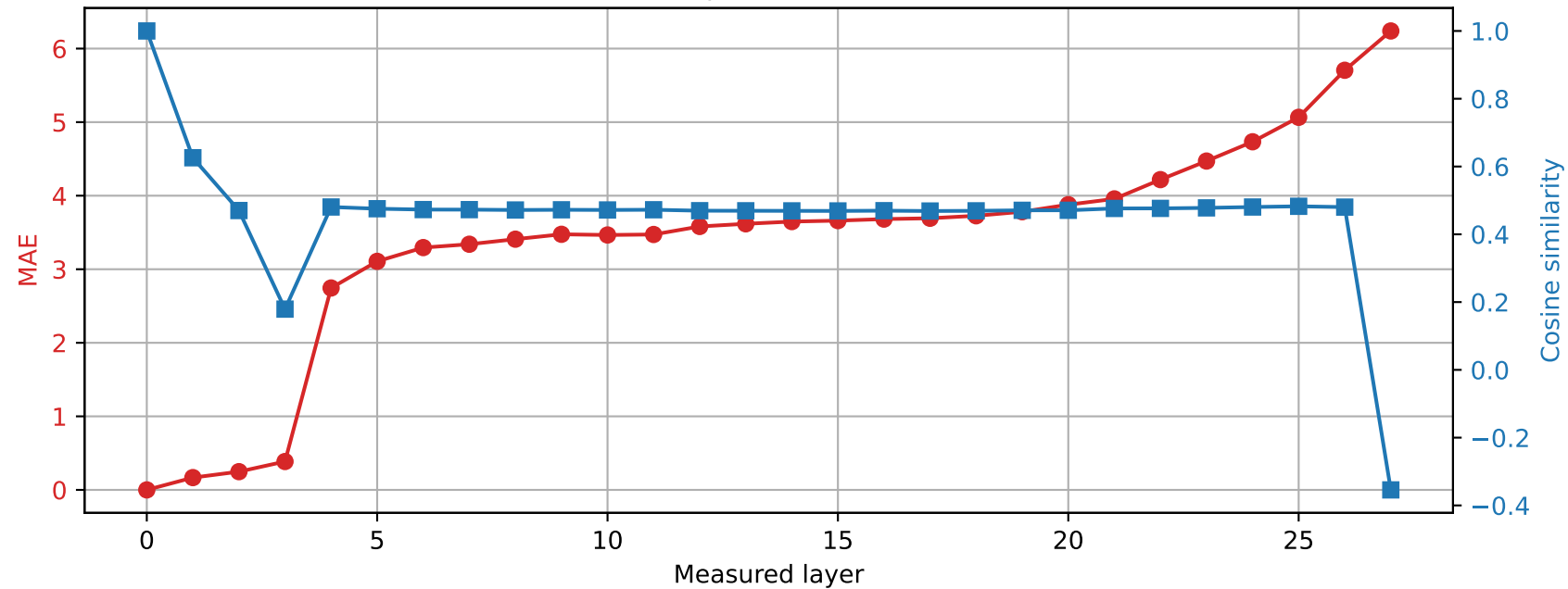
Qwen2.5-7B-Instruct | Prompt 2 Spared layer 5 | Hybrid vs unquantized
