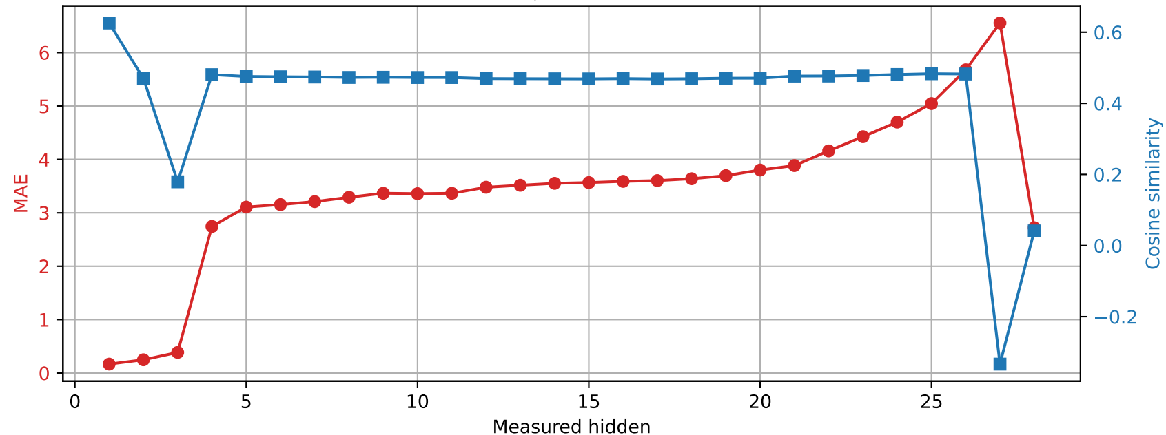
Qwen2.5-7B-Instruct | Prompt 2 Spared layer 10 | Unquantized vs hybrid
