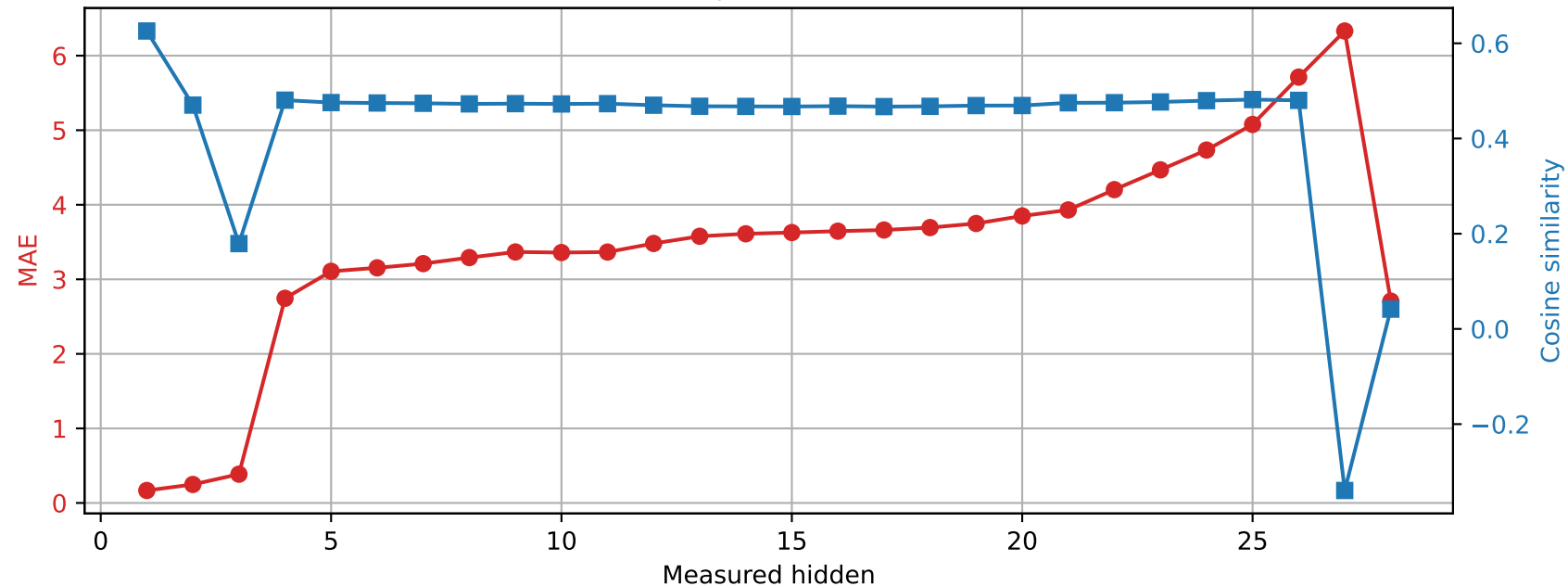
Qwen2.5-7B-Instruct | Prompt 2 Spared layer 12 | Unquantized vs hybrid
