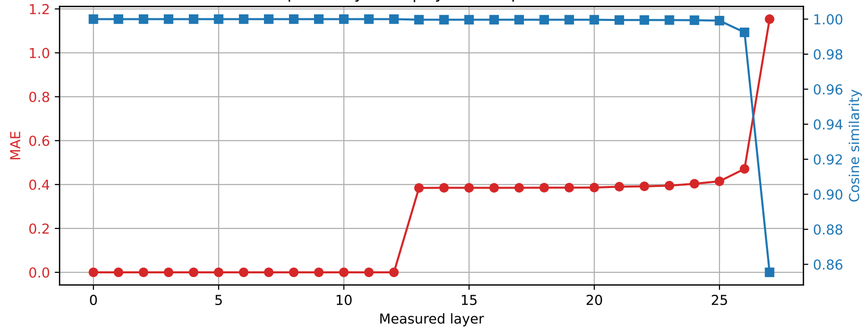
Qwen2.5-7B-Instruct | Prompt 2 Spared layer 12 | Hybrid vs quantized
