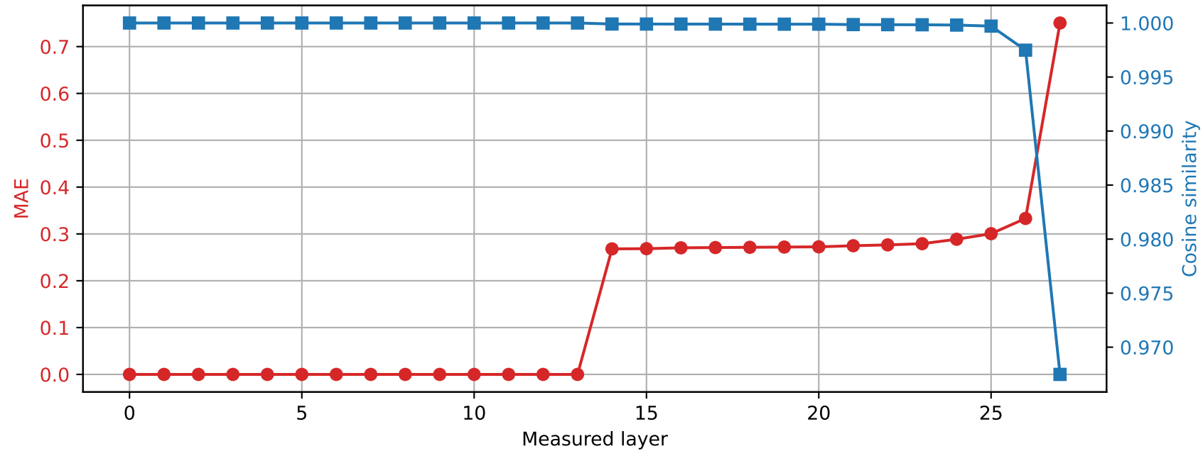
Qwen2.5-7B-Instruct | Prompt 2 Spared layer 13 | Hybrid vs quantized
