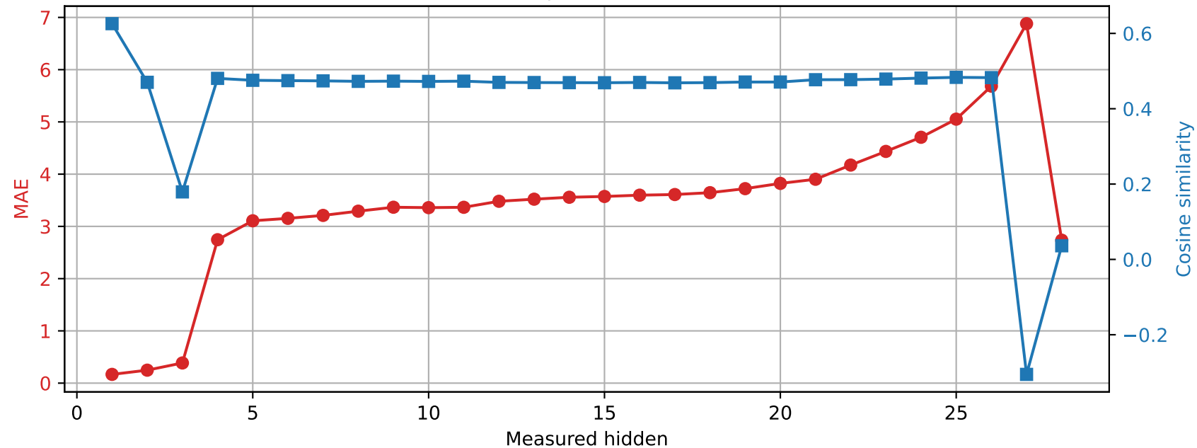
Qwen2.5-7B-Instruct | Prompt 2 Spared layer 18 | Unquantized vs hybrid
