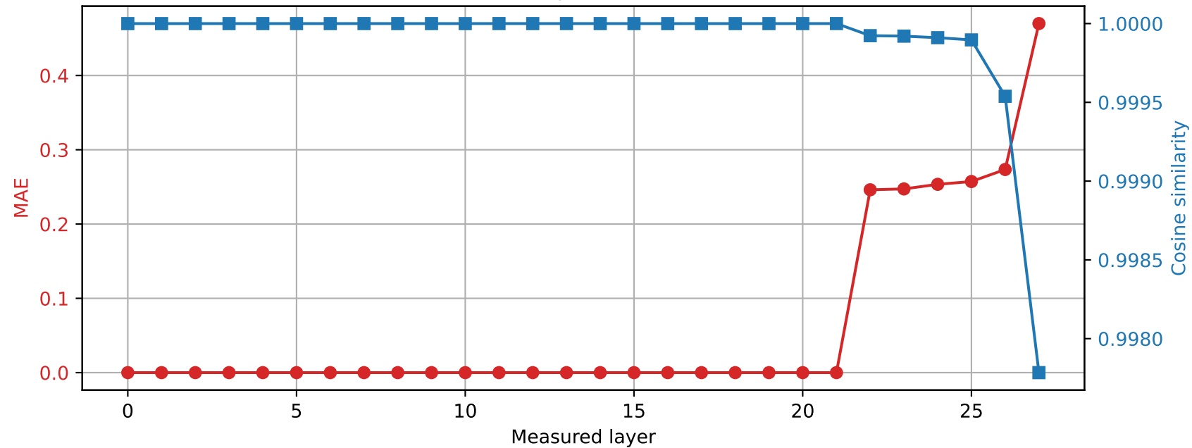
Qwen2.5-7B-Instruct | Prompt 2 Spared layer 21 | Hybrid vs quantized
