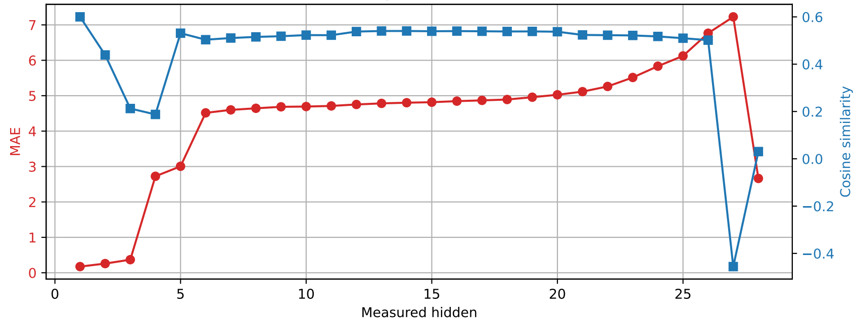
Qwen2.5-7B-Instruct | Prompt 3 Spared layer 5 | Unquantized vs hybrid
