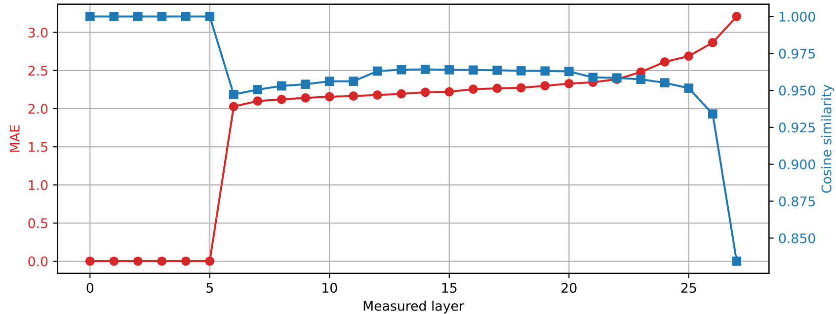
Qwen2.5-7B-Instruct | Prompt 3 Spared layer 5 | Hybrid vs quantized
