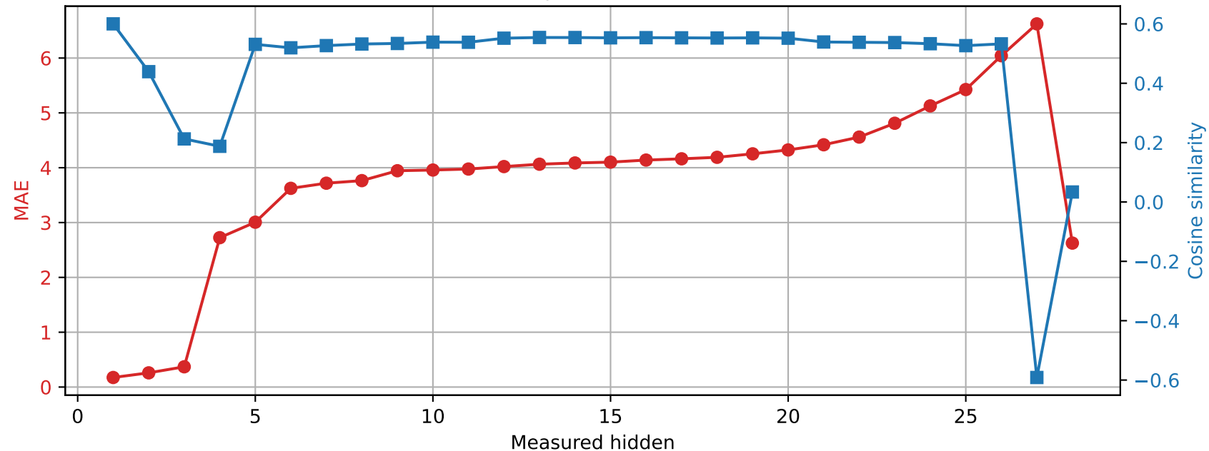
Qwen2.5-7B-Instruct | Prompt 3 Spared layer 8 | Unquantized vs hybrid
