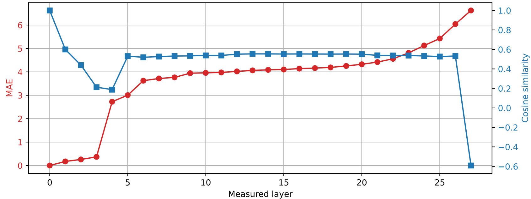
Qwen2.5-7B-Instruct | Prompt 3 Spared layer 8 | Hybrid vs unquantized
