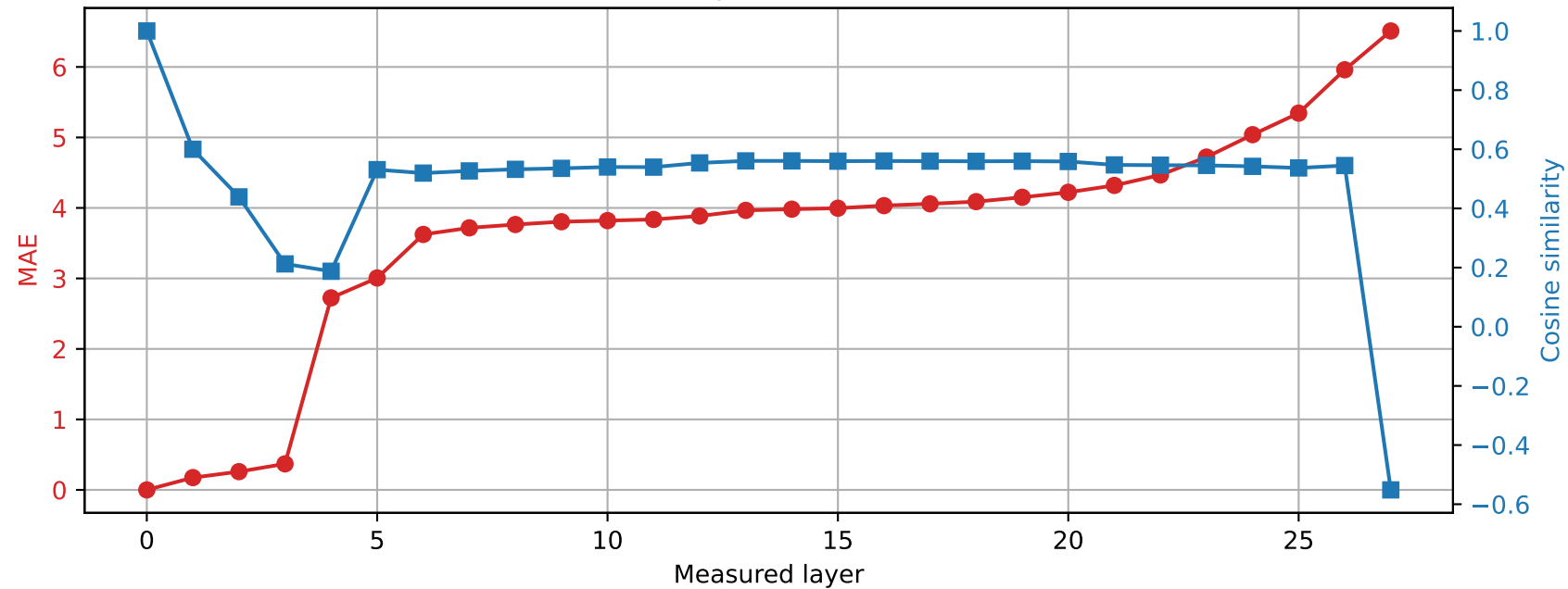
Qwen2.5-7B-Instruct | Prompt 3 Spared layer 12 | Hybrid vs unquantized
