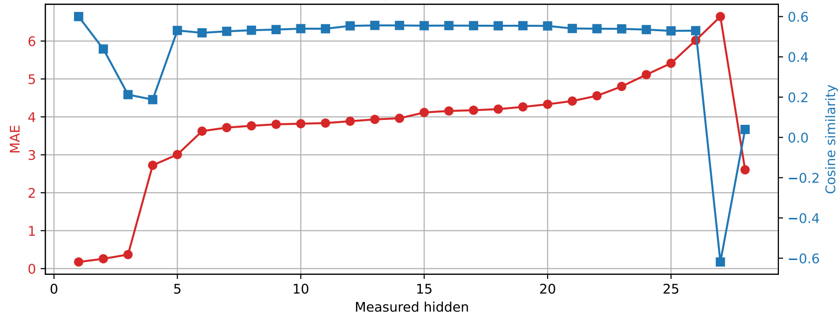
Qwen2.5-7B-Instruct | Prompt 3 Spared layer 14 | Unquantized vs hybrid
