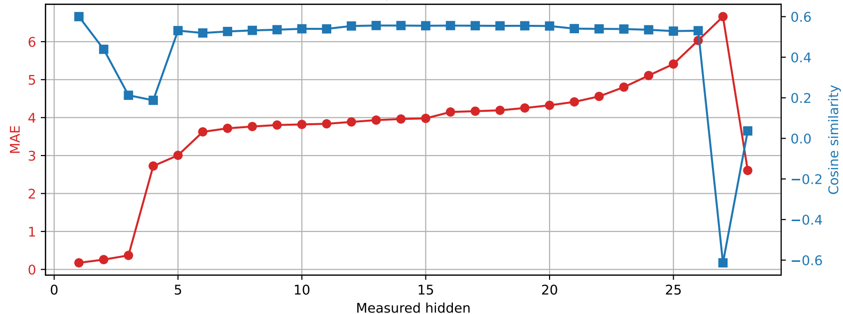
Qwen2.5-7B-Instruct | Prompt 3 Spared layer 15 | Unquantized vs hybrid
