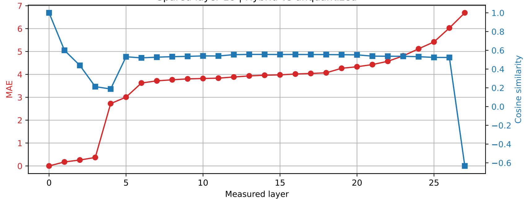
Qwen2.5-7B-Instruct | Prompt 3 Spared layer 18 | Hybrid vs unquantized
