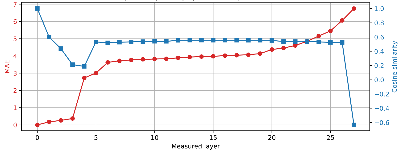
Qwen2.5-7B-Instruct | Prompt 3 Spared layer 19 | Hybrid vs unquantized
