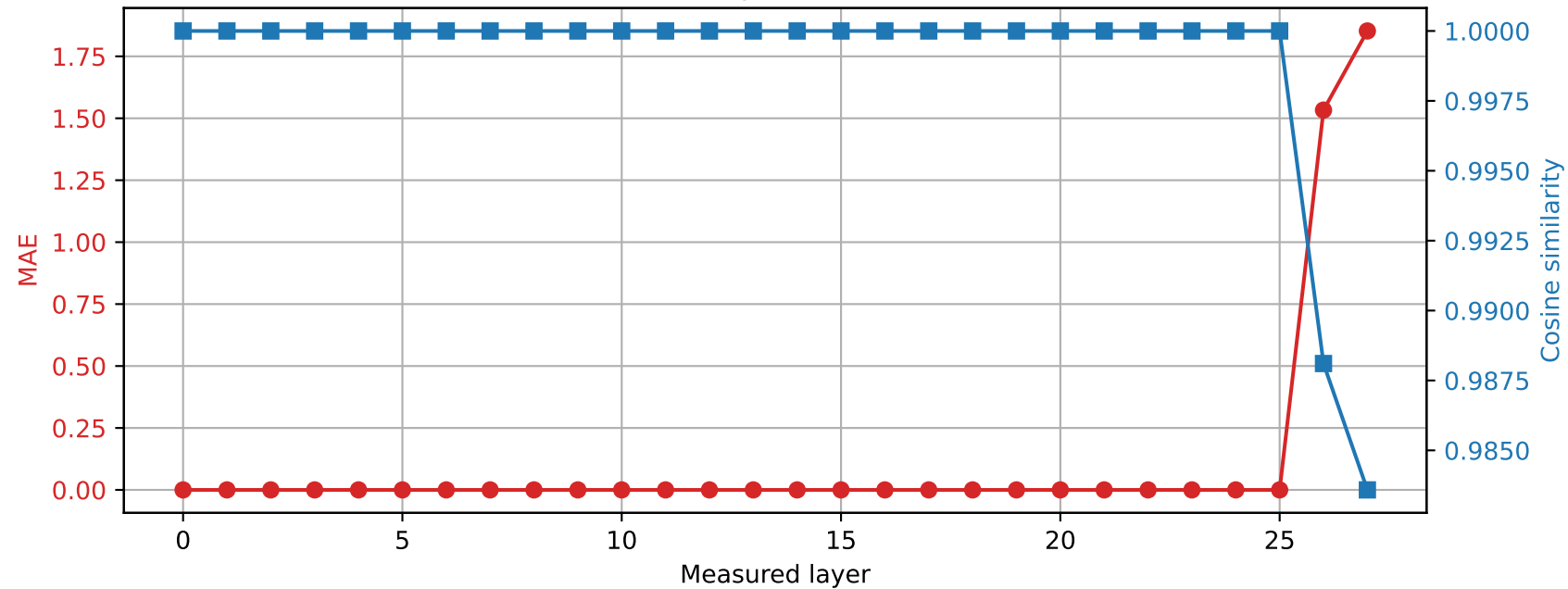
Qwen2.5-7B-Instruct | Prompt 3 Spared layer 25 | Hybrid vs quantized
